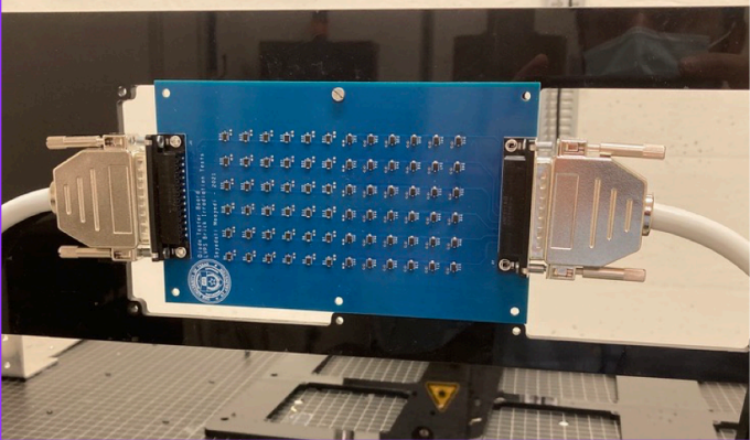
A diode test board in CC60 facility
