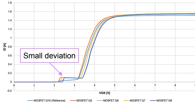
MOSFET Characterization at V_{DS} = 1V
