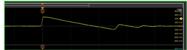
SET in LT3080 output voltage
