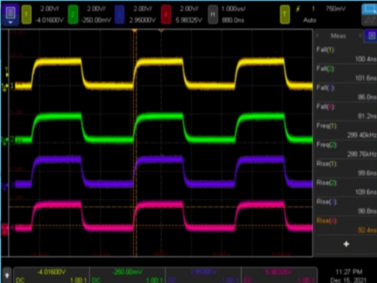
Output pulses of IR2110
