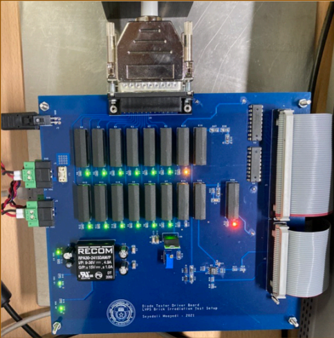
Relay board
