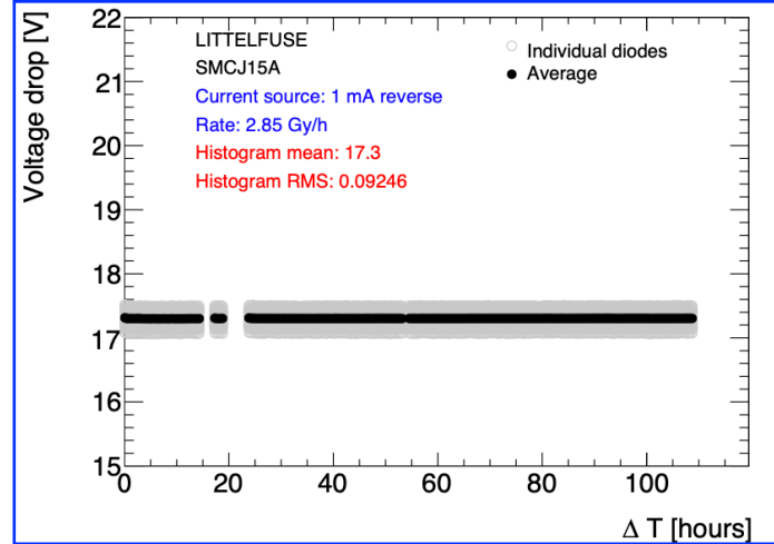
SMCJ15A breakdown voltage (During TID)
