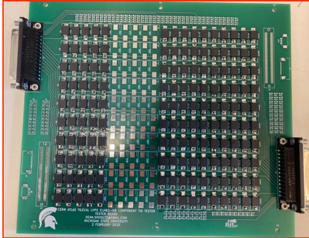
SMCJ15A test board
