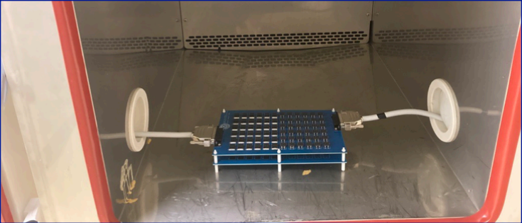
A diode test board inside climatic chamber
