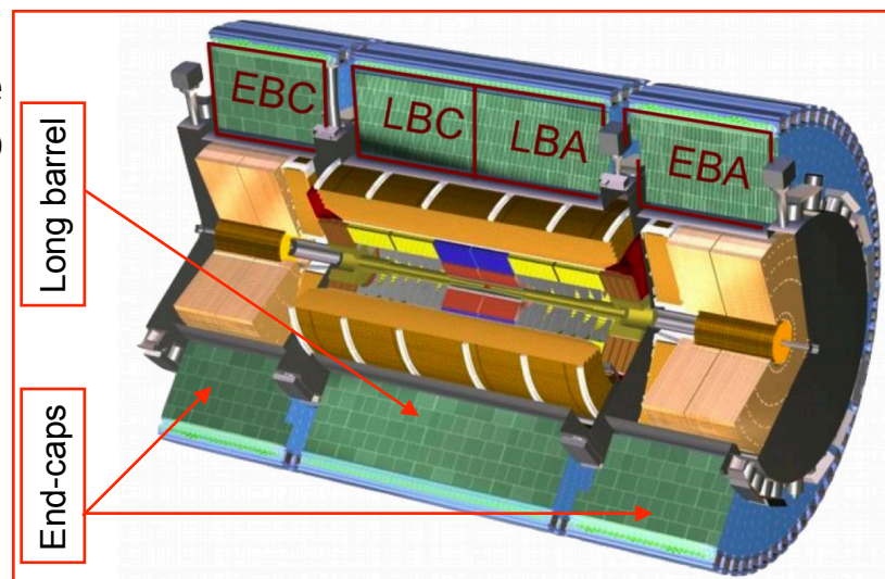
ATLAS Tile Calorimeter drawing
