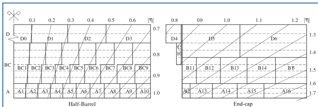
Mapping of Tile Calorimeter cells
