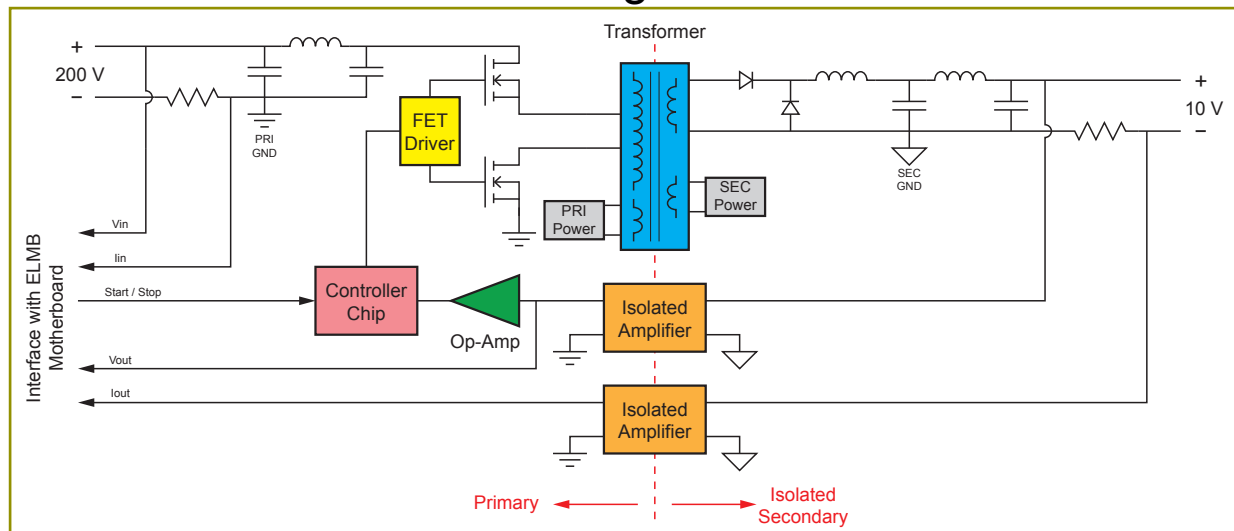
LVPS brick functional block diagram
