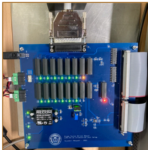
Relay board
