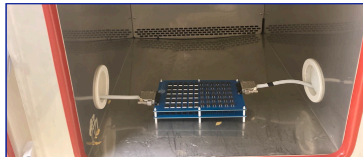
A diode test board inside climatic chamber
