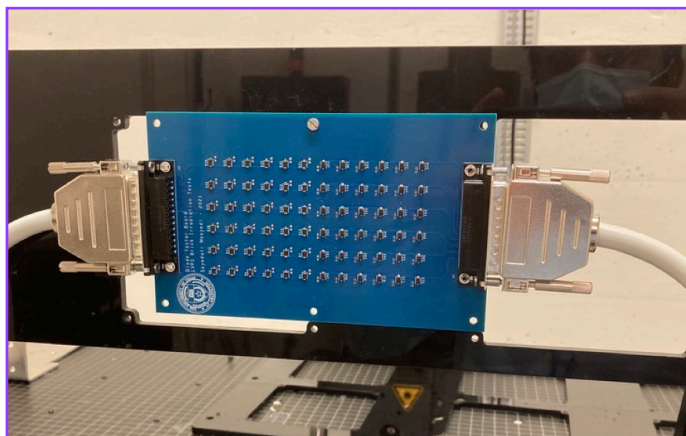
A diode test board in CC60 facility
