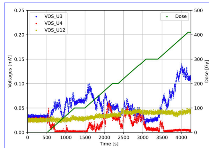
Offset voltage in LTC6241
