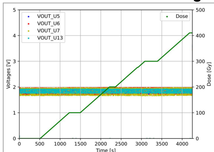
Output voltage in LTC6241
