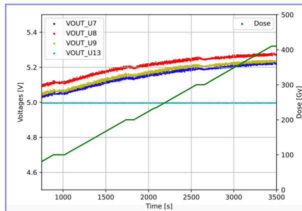
Output voltage of LT3080 during tests at PIF
