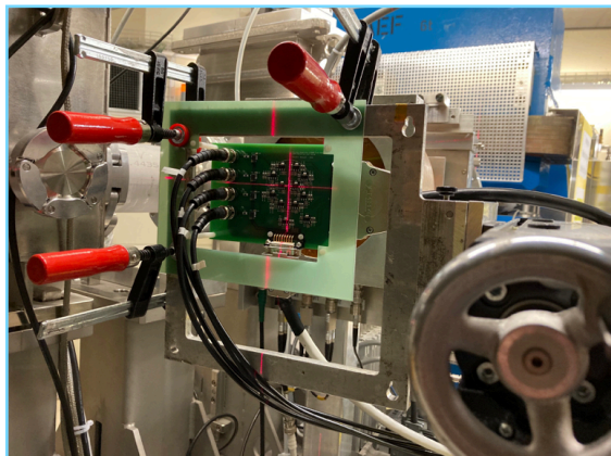
LT3080 test board at PIF
