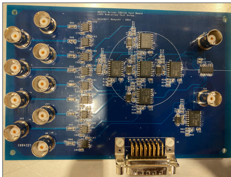
Designed board for testing IR2110
