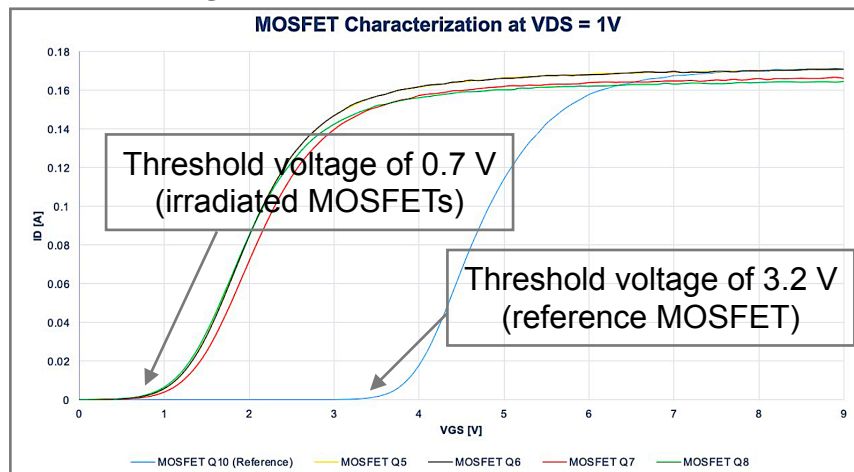
MOSFET characterization after TID of 200 Gy
