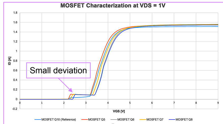
MOSFET characterization after NIEL tests
