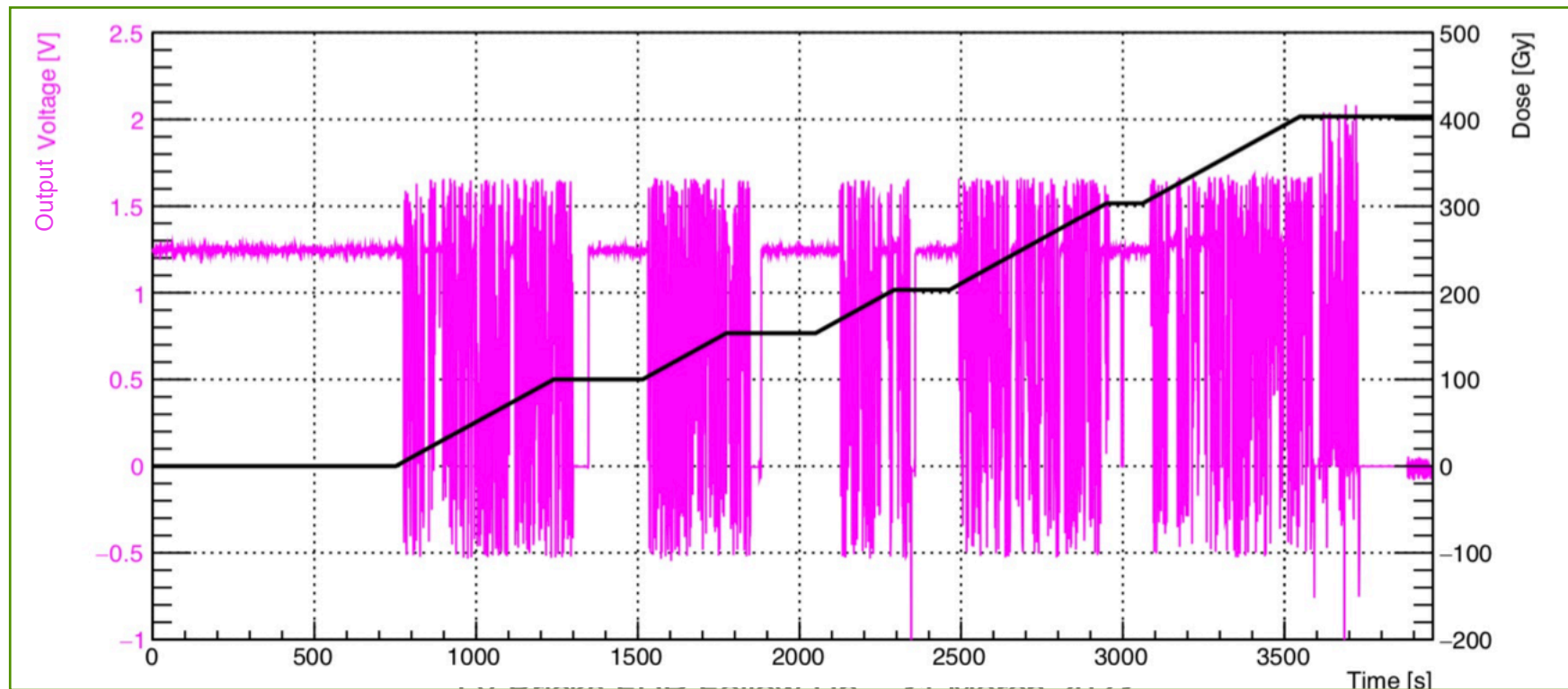
Unstable behavior of SI8920 at input voltage of 150 mV at PIF
