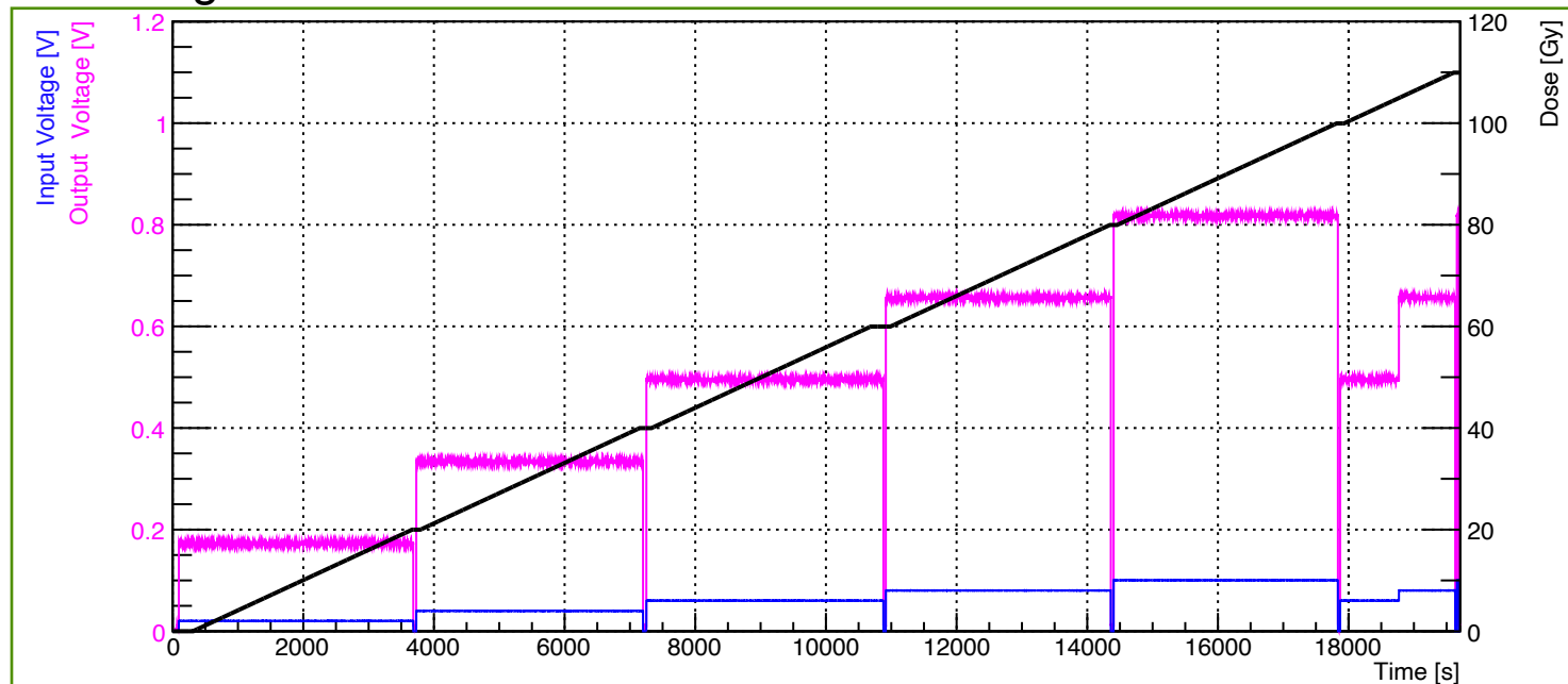
Stable behavior of SI8920 at input voltage below 100 mV at PIF
