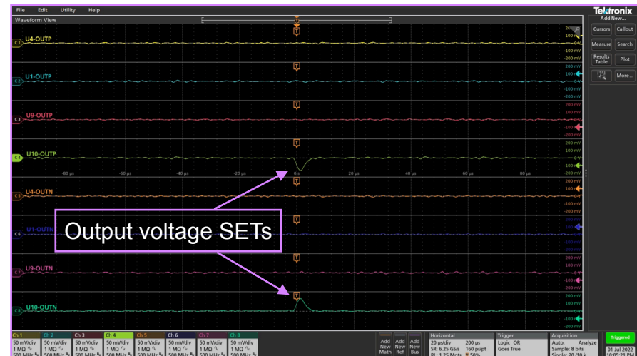
Couple of SETs in HCPL7800 output voltages
