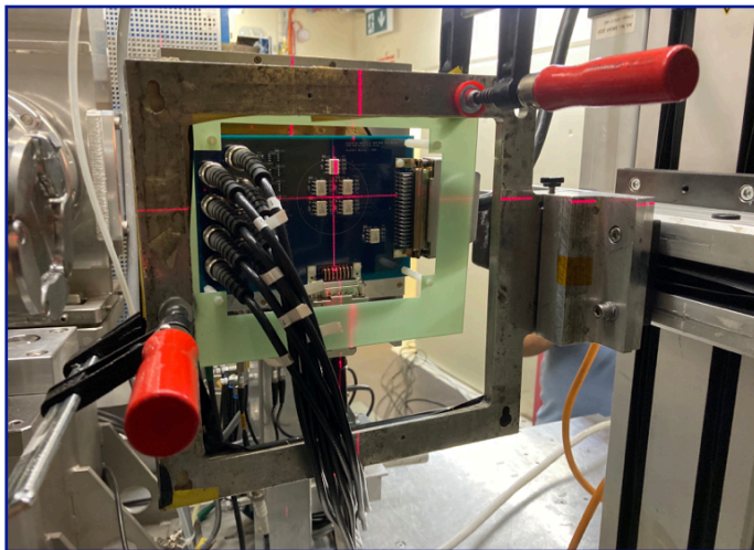
HCPL7800 test board at PIF
