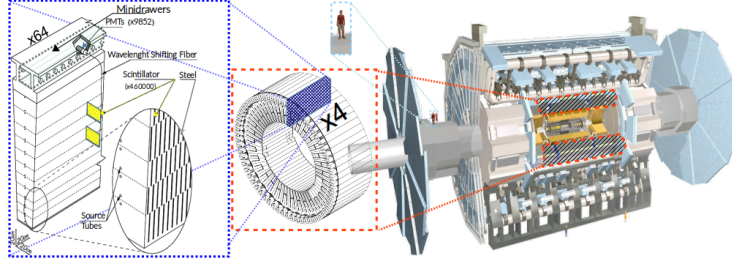
Figure 1 . TileCal structure in ATLAS.
