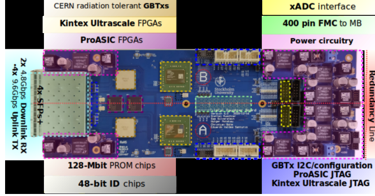
Figure 2 . The DB6 layout.
