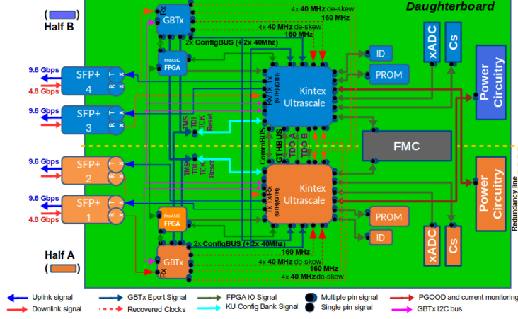
Figure 2 . The Daughterboard revision 6 block diagram.
