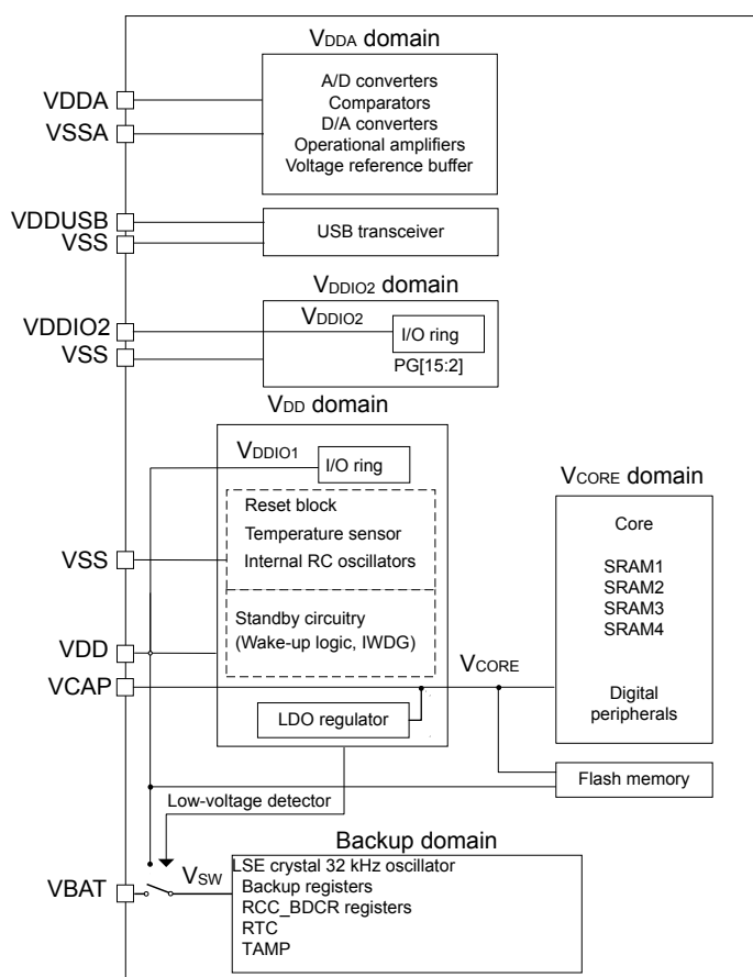
Figure 2. STM32U3B5xx power supply overview (without SMPS)
