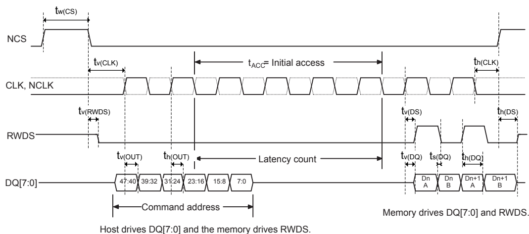
Figure 52. OCTOSPI HyperBus read with double latency
