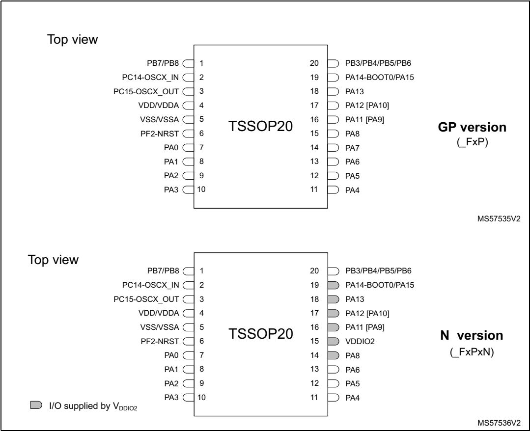
Figure 4. STM32C071FxFP TSSOP20 pinout
