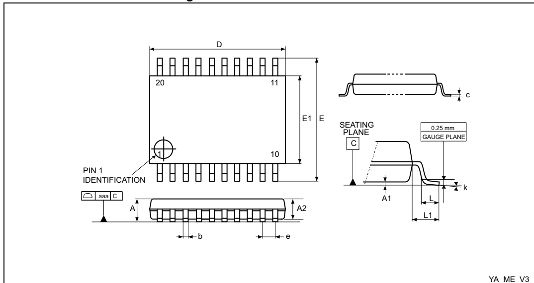
Figure 35. TSSOP20 – Outline
