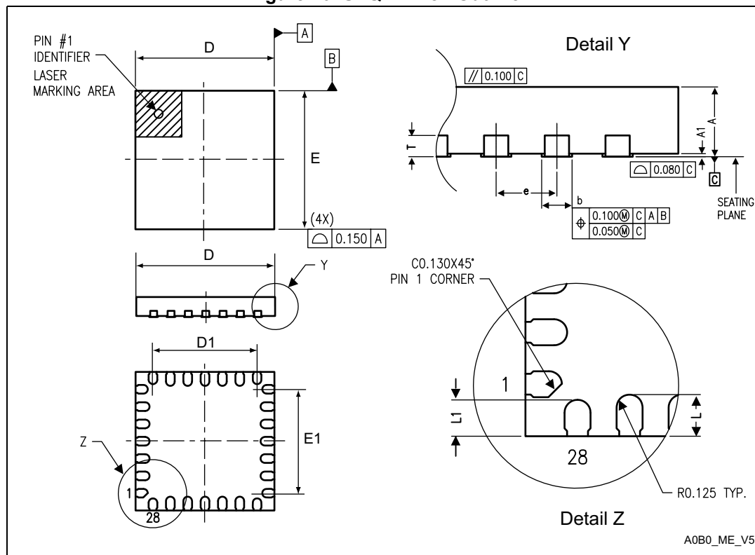
Figure 40. UFQFPN28 - Outline
