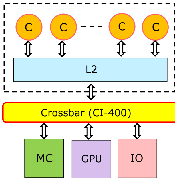
Symmetrical multicore
