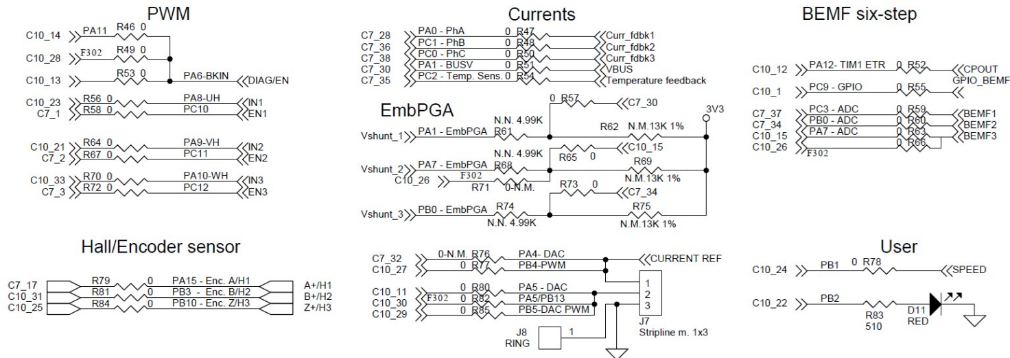
Figure 4. X-NUCLEO-IHM07M1 circuit schematic (4 of 4)
