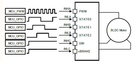
Figure 18. 1x PWM—Simple Controller
