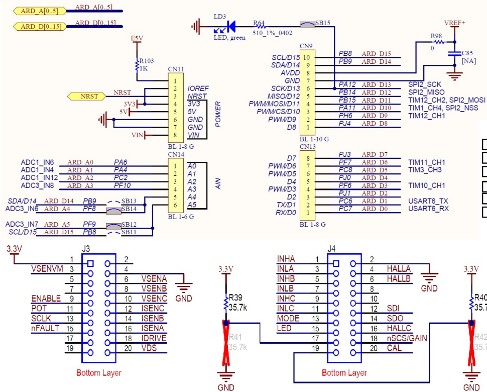
Figure 18. 1x PWM—Simple Controller
