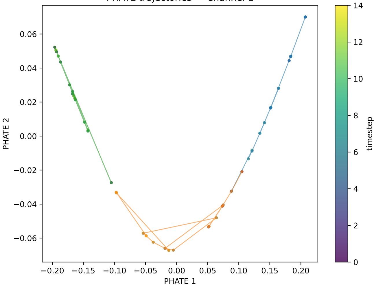
PHATE trajectories — Channel 1
