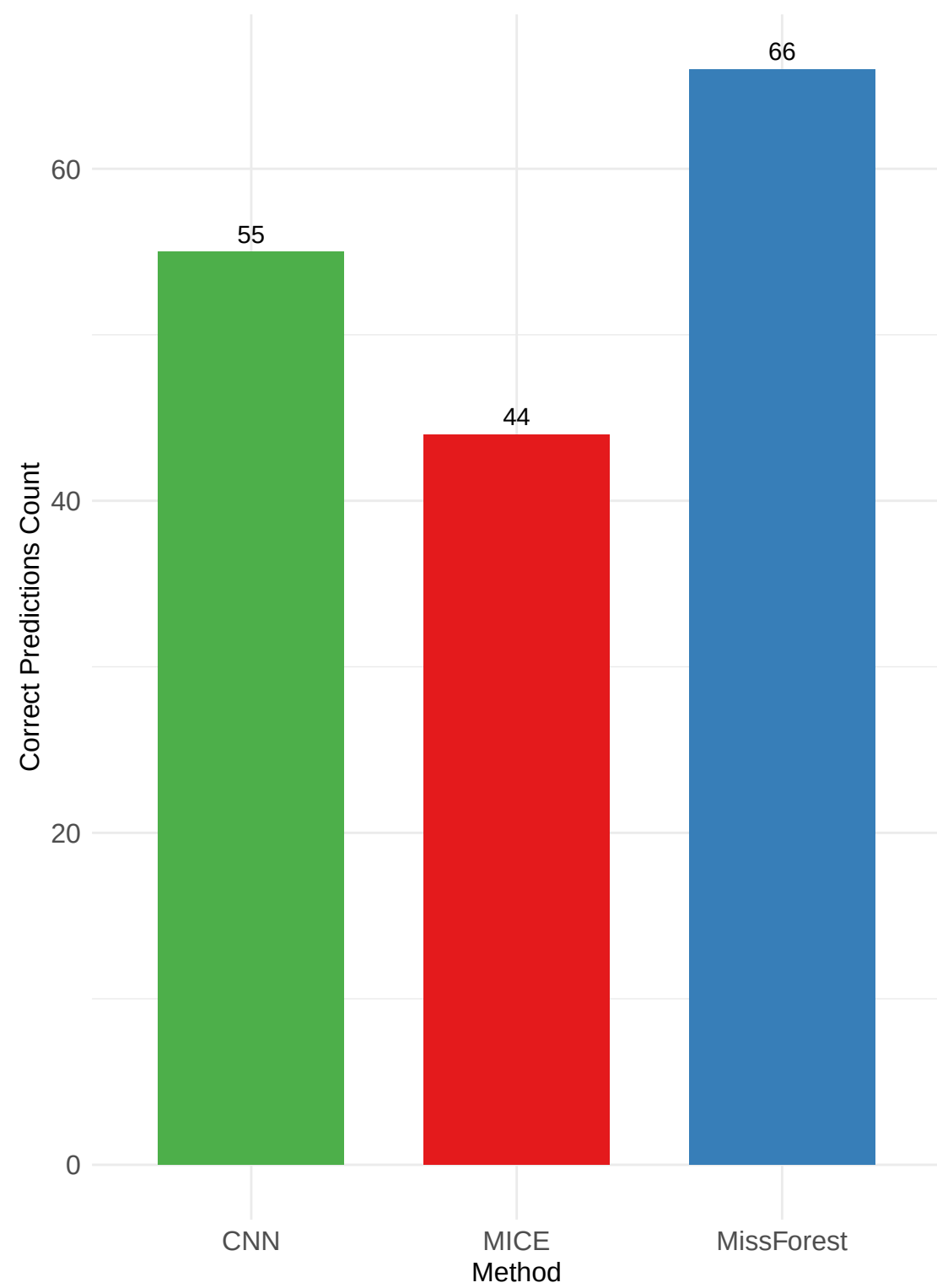
Method-wise Correct Predictions Count
