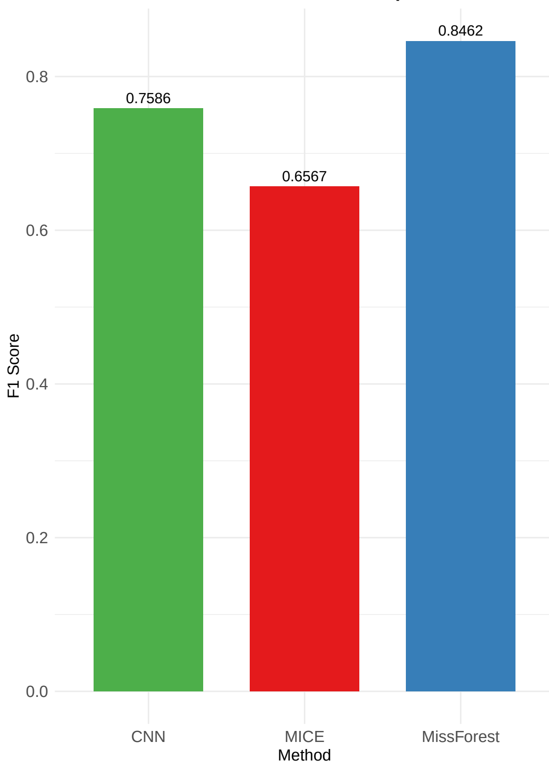
Method-wise F1 Score Comparison
