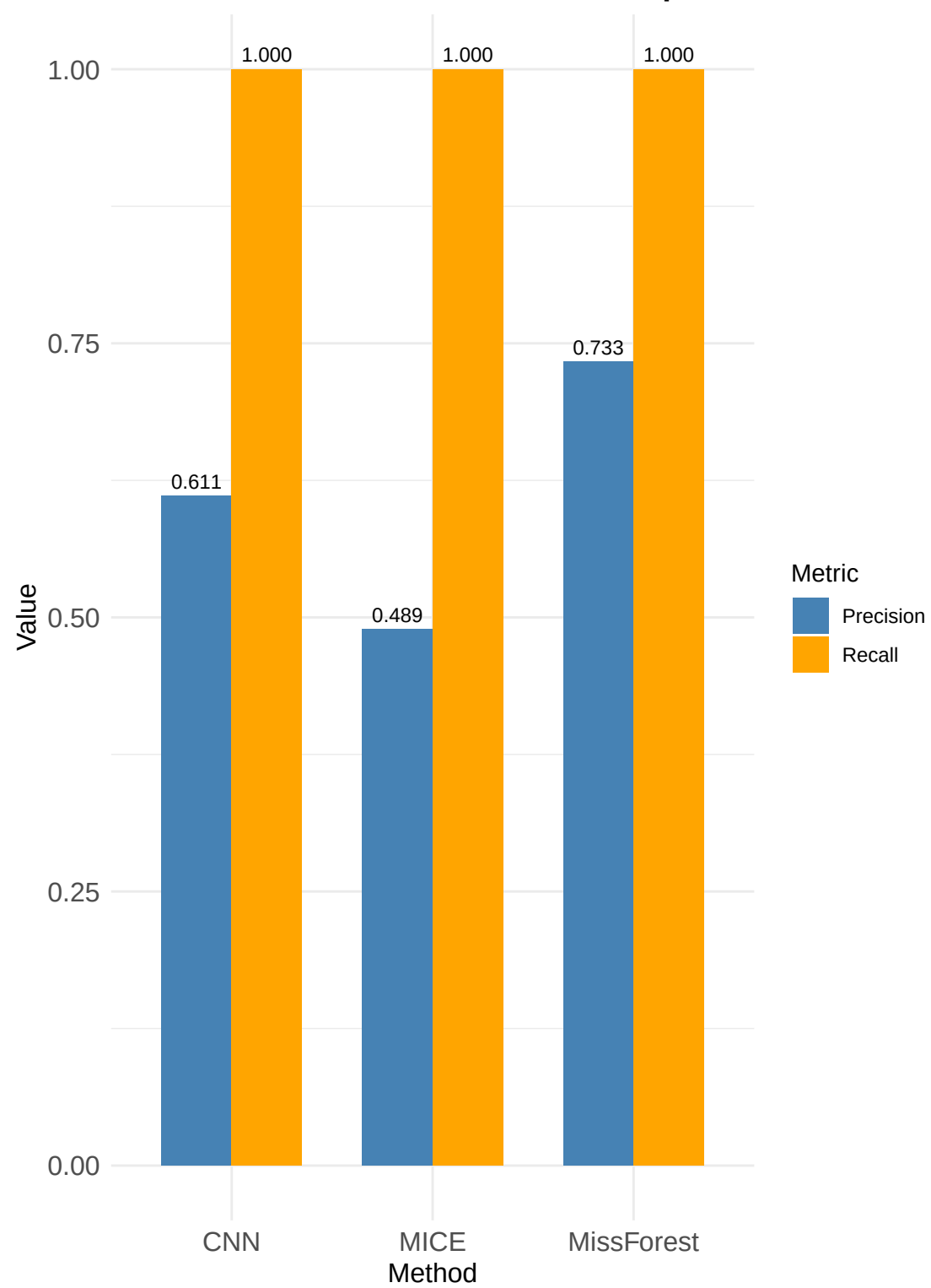
Method-wise Precision vs Recall Comparison
