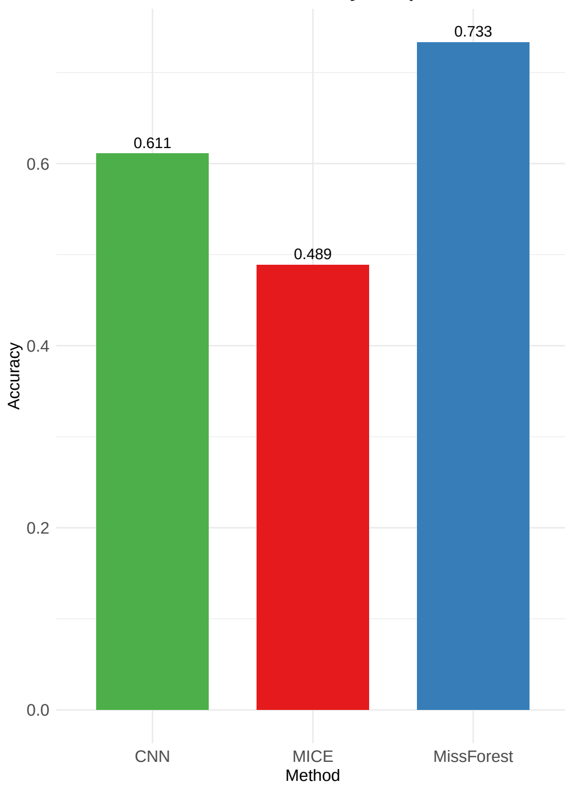
Method-wise Accuracy Comparison
