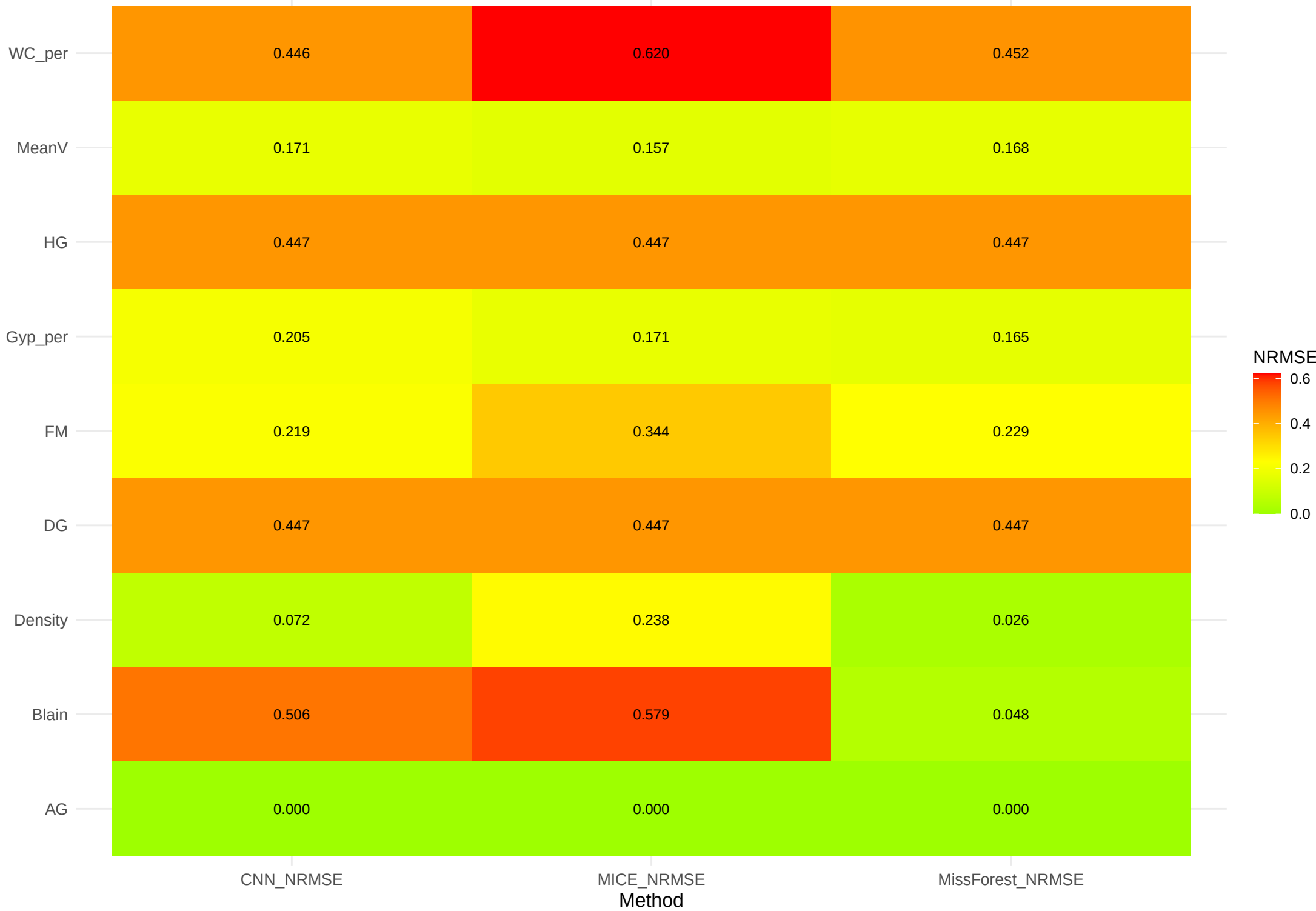
NRMSE Heatmap for Numeric Data
