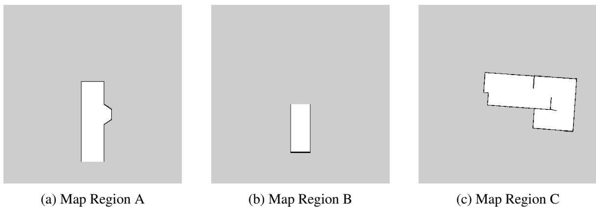
Gambar 3.4: Map Occupancy Grid masing-masing region
