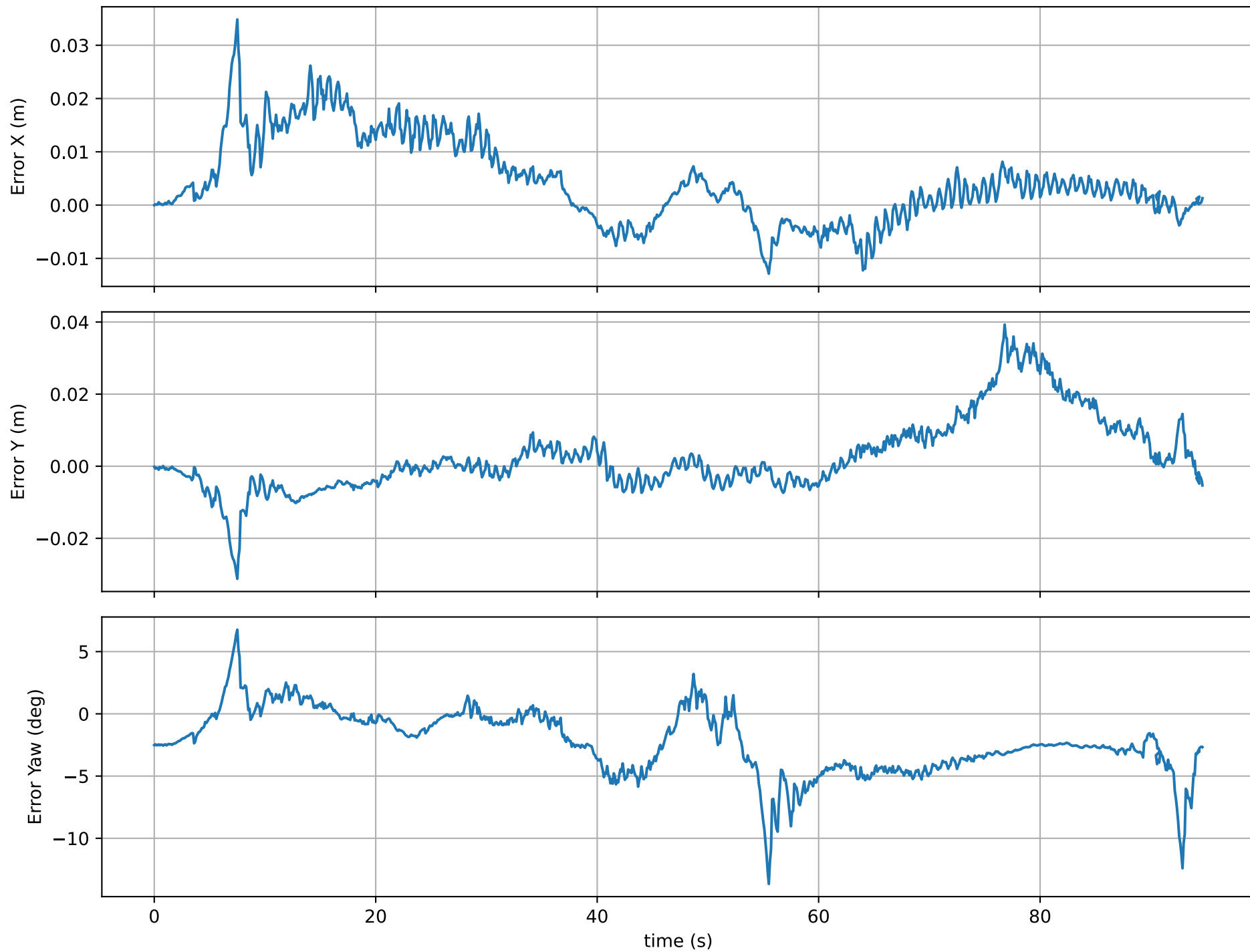
ICP Error over Time
