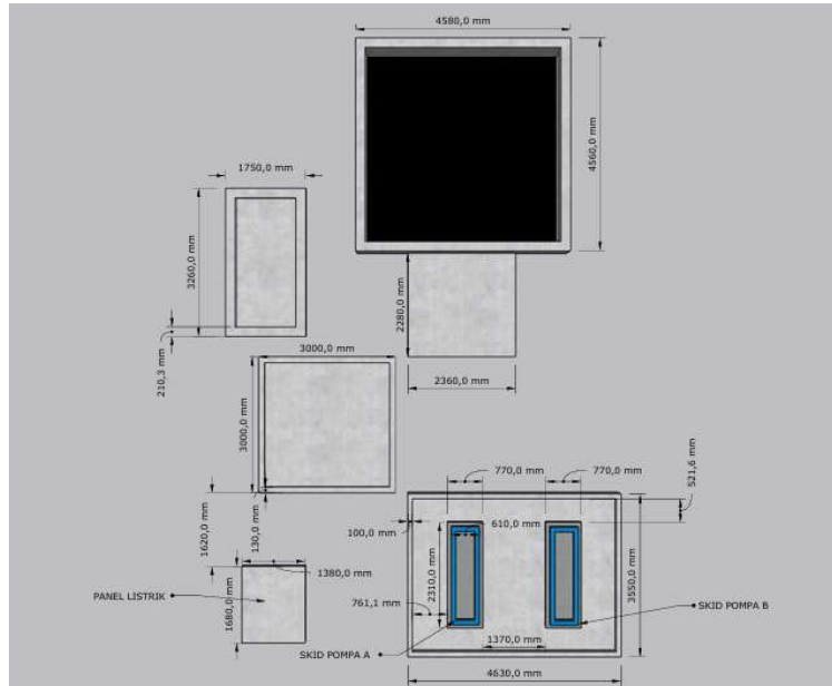
Gambar 8.1. Layout Fondasi Sump Pump Area 5NW
