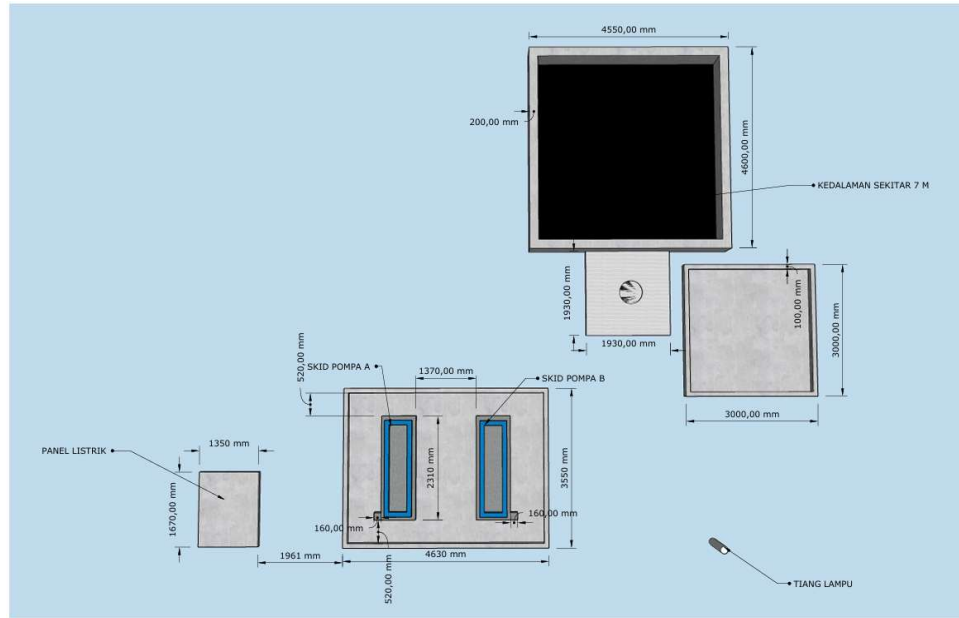
Gambar 8.1. Layout Fondasi Sump Pump Area 5SW
