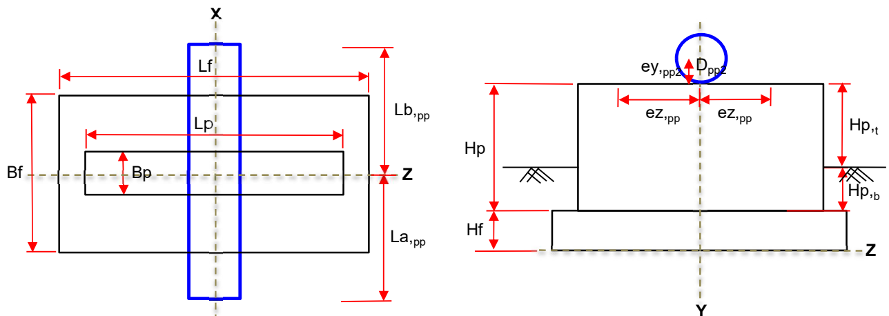
Dimensi Pipe SLEEPER - Pipe Support CGS-1 Tipe 1B
