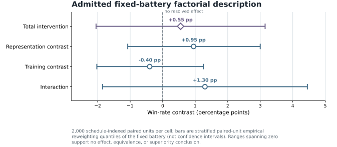
FIG. 5. Prespecified fixed-battery factorial contrasts and the 2.5th and 97.5th percentiles from the prespecified stratified paired-unit resampling algorithm, reported as empirical reweighting for 2,000 schedule-indexed units. The bars are descriptive sensitivities, not confidence intervals, equivalence tests, or statements about new opponents, seeds, or training runs. Source data are in source_data/figure_5_factorial.csv .
