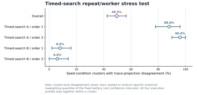
FIG. 4. Fixed-battery trace-projection disagreement in the timed-search stress test. Bars show descriptive empirical reweighting quantiles; all four execution profiles stay together within a cluster, while stratum results make the context heterogeneity visible. These quantiles are not confidence intervals. Any mismatch rejects exact parity on the exercised schedule. Neutral labels replace package names. Source data are in source_data/figure_4_timed_search.csv .
