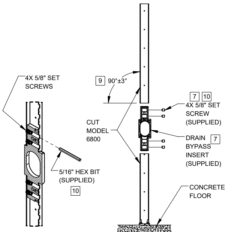
SECTION VIEW OF INSTALLED 6810W DRAIN BYPASS INSERT
