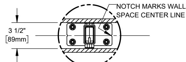
DETAIL D
