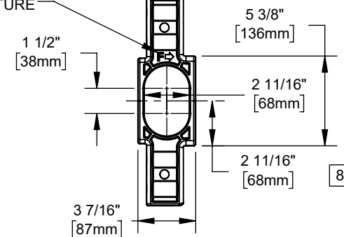
DRAIN BYPASS INSERT
