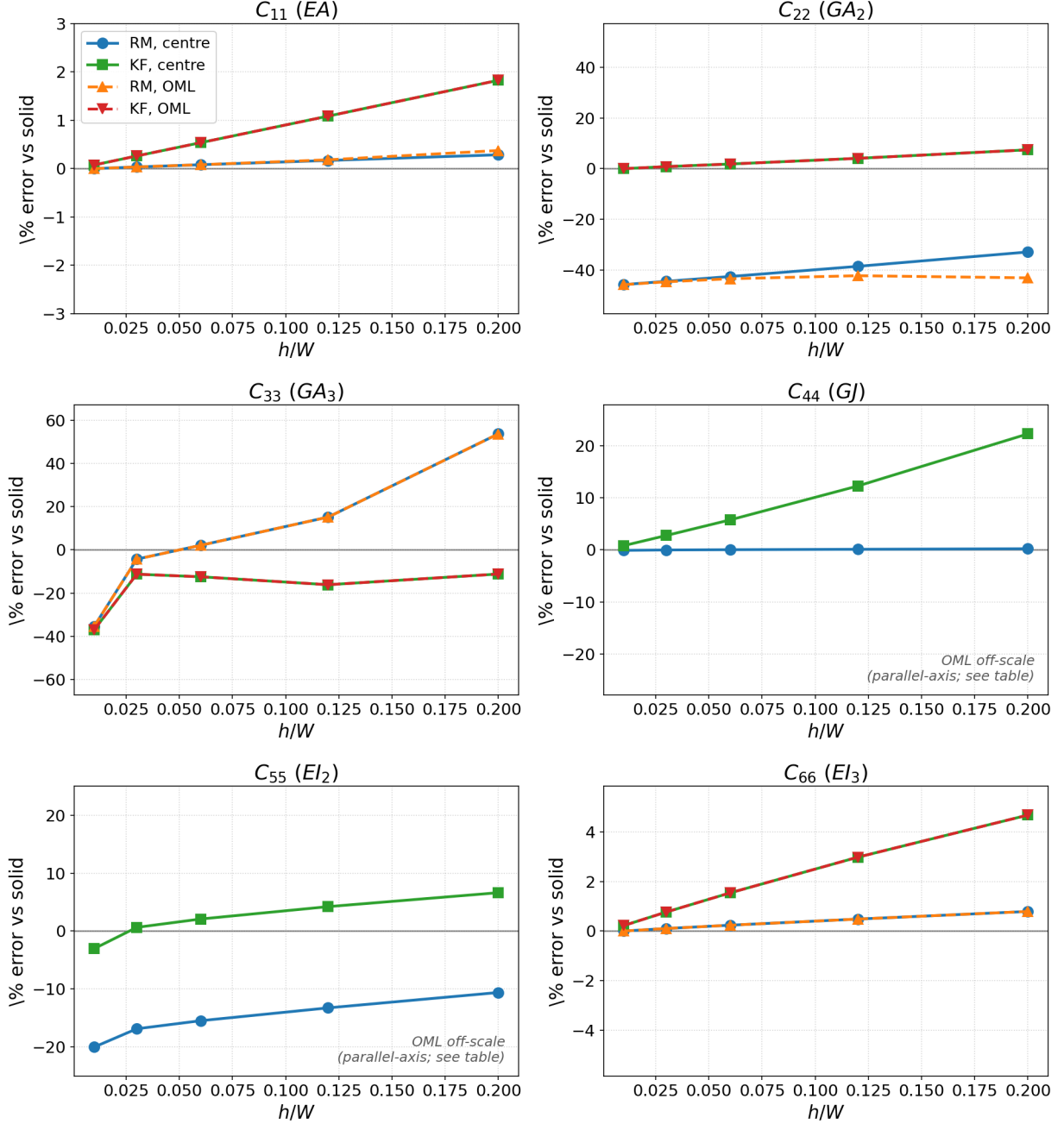
Figure 6: Anisotropic [45/−45] strip: % error vs. the solid. C_{44} ( GJ ): RM exact, KF rising to +22%. C_{22} ( GA_2 ): KF within 7%, RM \approx -40\% (converged RM open-section residual). C_{33} ( GA_3 ): off for both (1D limit). C_{55} ( El_2 ): RM soft (bend-twist), KF closer.
