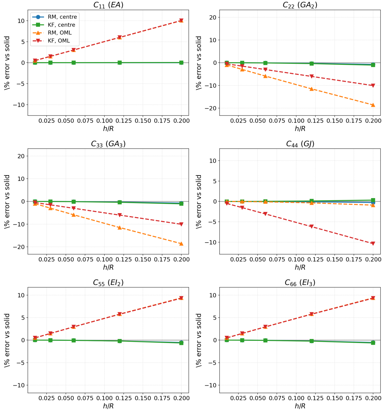
Figure 3: Isotropic tube: \% error vs. the solid for each Timoshenko component. Centre-reference curves (solid lines) hug zero through the thick range; OML (dashed) drifts O(h/R) .
