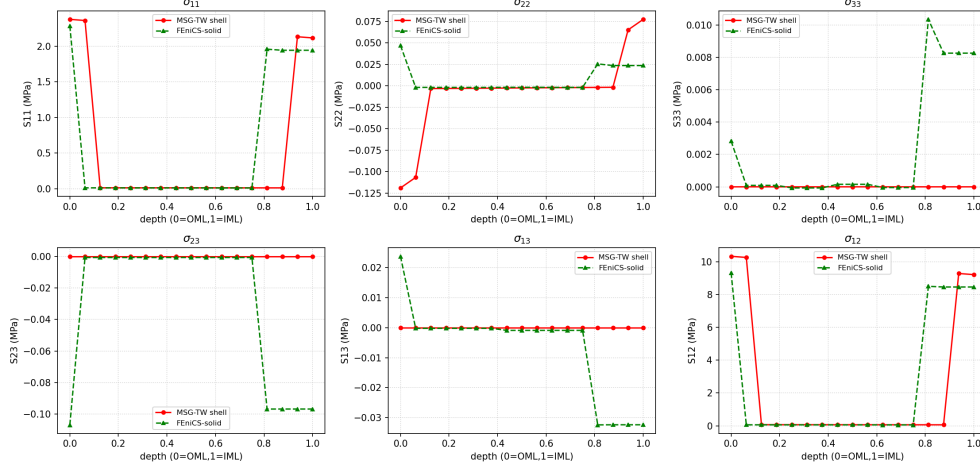
Figure 9: Station-13 recovered 3D stress (material frame) through the fore sandwich panel (44 mm), shell 1Dshell_13 vs FEniCS-solid, under a bending–torsion load. The axial stress \sigma_{11} (skins) matches to +4% and the torsional shear \sigma_{12} to +11%; the foam core is near stress-free. The small \sigma_{23} in the solid is the transverse shear the Kirchhoff recovery omits.
