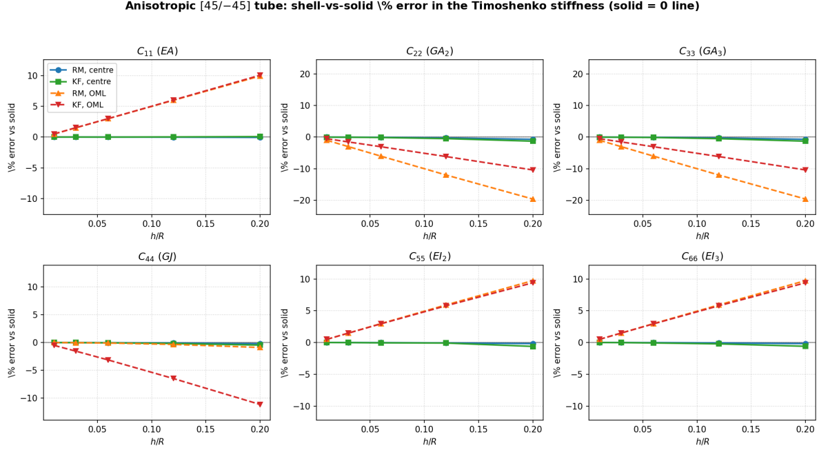
Figure 4: Anisotropic [45/−45] tube: % error vs. the solid. Same behaviour as the isotropic tube; < 1\% at the centre for both models across h/R .
