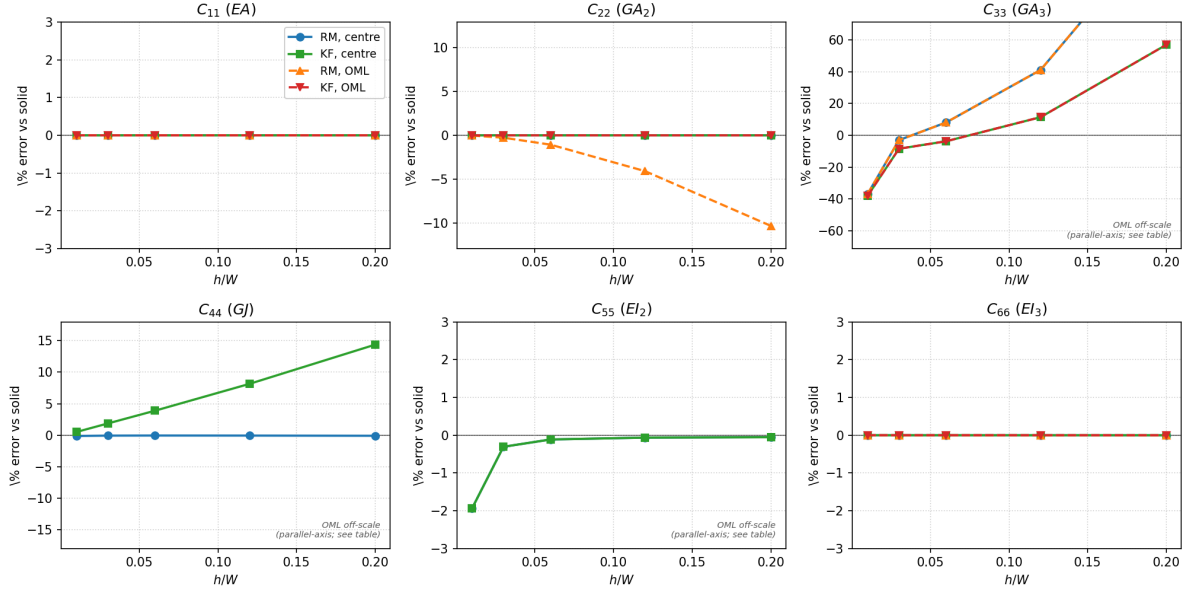
Figure 5: Isotropic strip: \% error vs. the solid. EA , EI_3 exact; GJ exact for RM and +0.5–14% for KF; EI_2 within 2% for both; GA_3 off for both (1D-shell limit). OML EI_2/GJ are reference offsets (off-scale).
