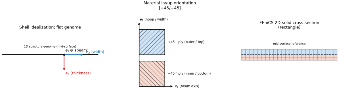
Figure 2: Plate-strip . Left: the flat 1D genome with the local frame ( e_2 along the width, e_3 through the thickness). Centre: the same [+45/−45] orientation. Right: the matching FEniCS 2D-solid rectangle. The strip is an open section (free edges), unlike the closed tube.
