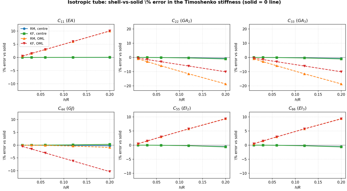
Figure 3: Isotropic tube: % error vs. the solid for each Timoshenko component. Centre-reference curves (solid lines) hug zero through the thick range; OML (dashed) drifts O(h/R) .
