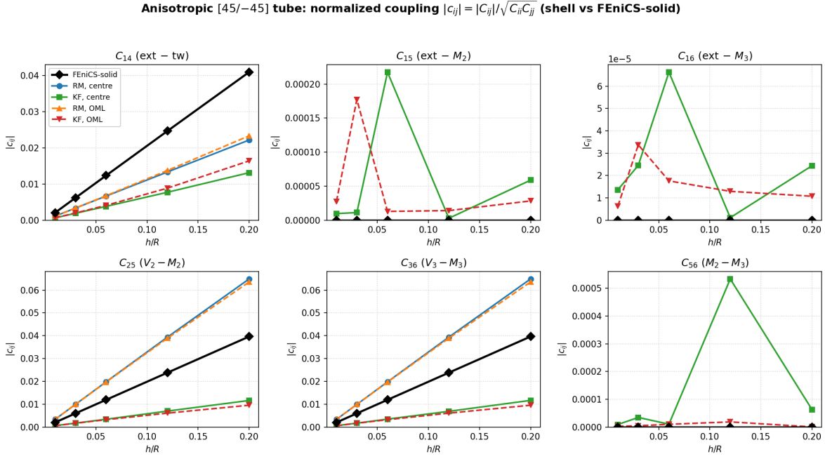
Figure 7: Anisotropic [45/−45] tube : normalized couplings vs. the solid. Genuine C_{14}, C_{25}, C_{36} \approx 0.04 (suppressed by closure); C_{15}, C_{16}, C_{56} \approx 0 .
