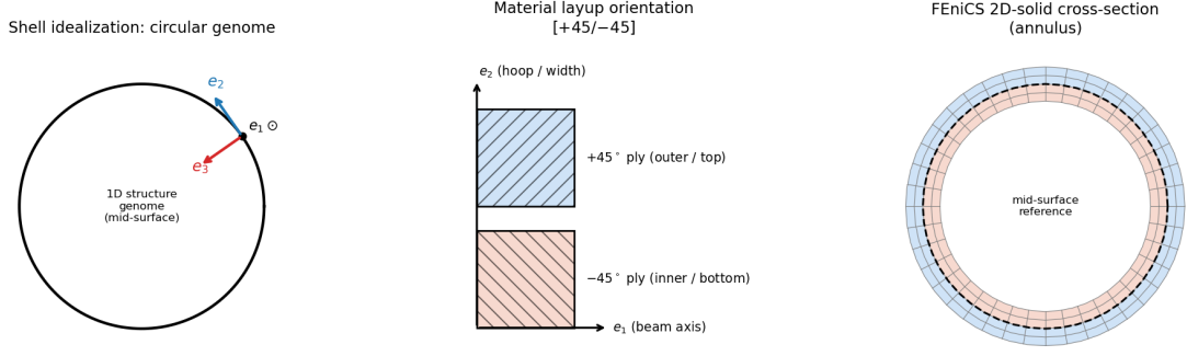
Figure 1: Tube . Left: the 1D shell genome (mid-surface circle) with the local frame e_1 (beam, out of plane), e_2 (hoop), e_3 (through-thickness). Centre: the [+45/−45] material orientation (fiber tows shown in each ply, relative to e_1/e_2 ). Right: the matching FEniCS 2D-solid annulus with the two ply bands and the mid-surface reference.
