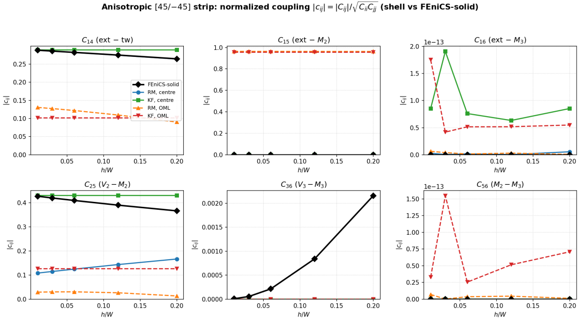
Figure 8: Anisotropic [45/−45] strip : C_{14} ( \approx 0.29 , captured by both models) and C_{25} ( \approx 0.43 , captured by KF, under-predicted by RM) are the genuine couplings; C_{15} is the OML parallel-axis artifact; C_{16}, C_{36}, C_{56} \approx 0 .
