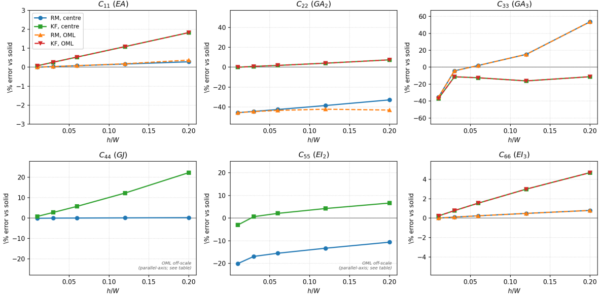
Figure 6: Anisotropic [45/-45] strip: % error vs. the solid. C_{44} ( GJ ): RM exact, KF rising to +22%. C_{22} ( GA_2 ): KF within 7%, RM \approx -40\% (converged RM open-section residual). C_{33} ( GA_3 ): off for both (1D limit). C_{55} ( EI_2 ): RM soft (bend-twist), KF closer.
