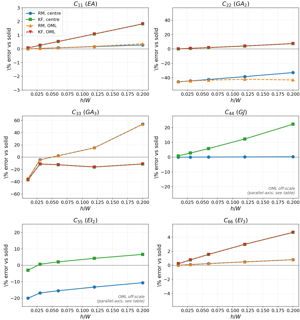
Figure 1: [45/−45] strip: \% error vs. the solid (centre = solid lines, OML = dashed). Note C_{44} ( GJ ): RM flat at zero, KF rising to +22%—RM is more accurate for thick open-section torsion. C_{33} ( GA_3 ) is off for both (1D-shell limit); C_{22} ( GA_2 ) is under-predicted by RM. OML EI_2/GJ are off-scale reference offsets. (Full set of error/coupling plots in benchmark_report.pdf .)
