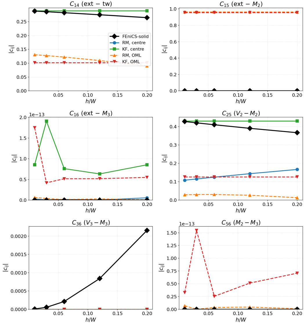
Figure 2: [45/−45] strip normalized couplings |c_{ij}| . C_{14} (ext-twist) and C_{25} (shear-bend) are the genuine material couplings; C_{15} is the OML parallel-axis artifact; C_{16}, C_{36}, C_{56} \approx 0 .
