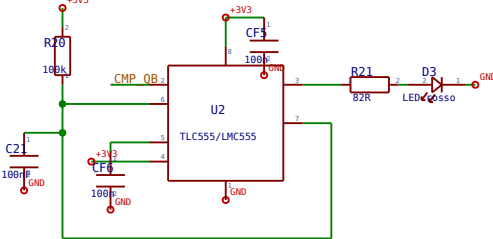
Monostabile LED (~11ms)
