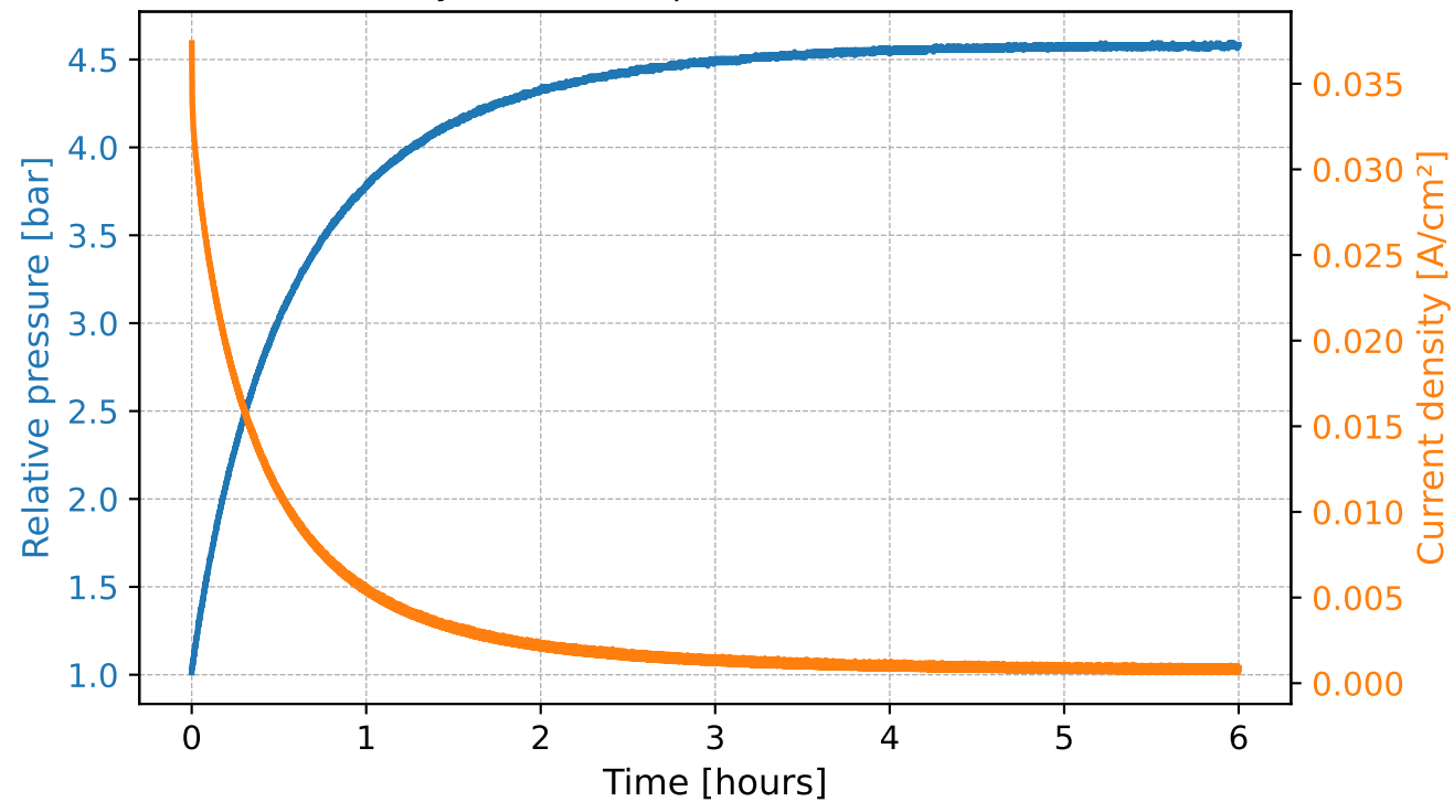
Current density vs Relative pressure of the cathode - 0.02 V
