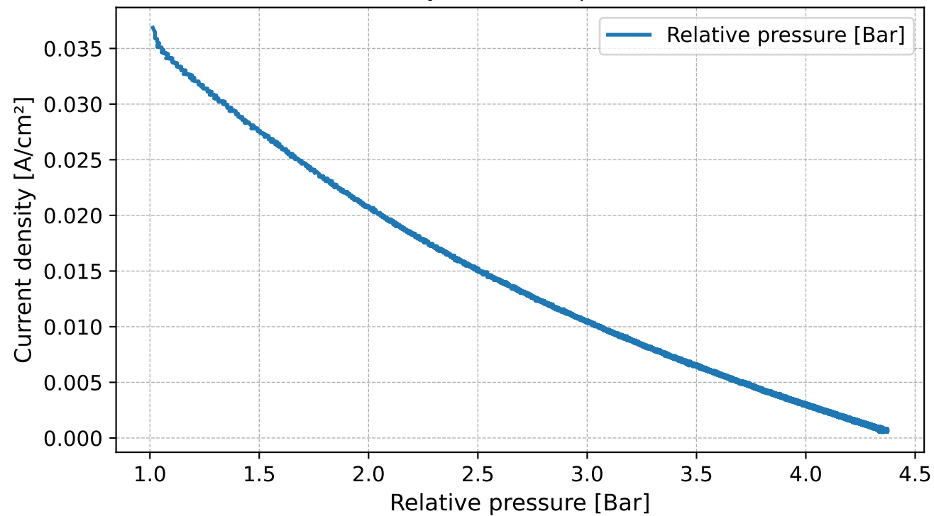
Current density vs Relative pressure - 0.02 V
