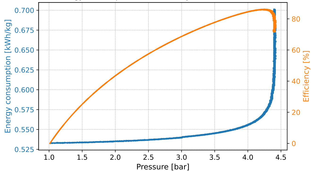
Energy consumption and efficiency vs Pressure - 0.02 V
