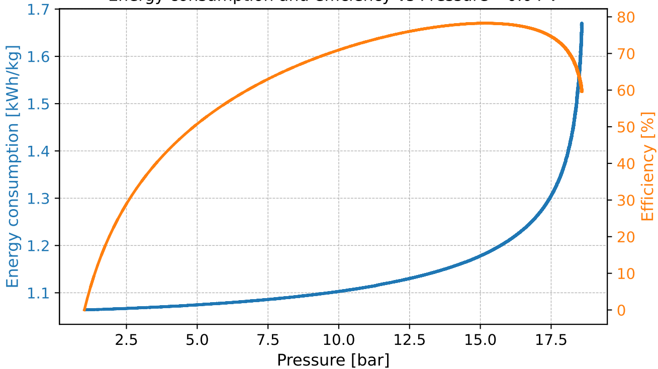
Energy consumption and efficiency vs Pressure - 0.04 V
