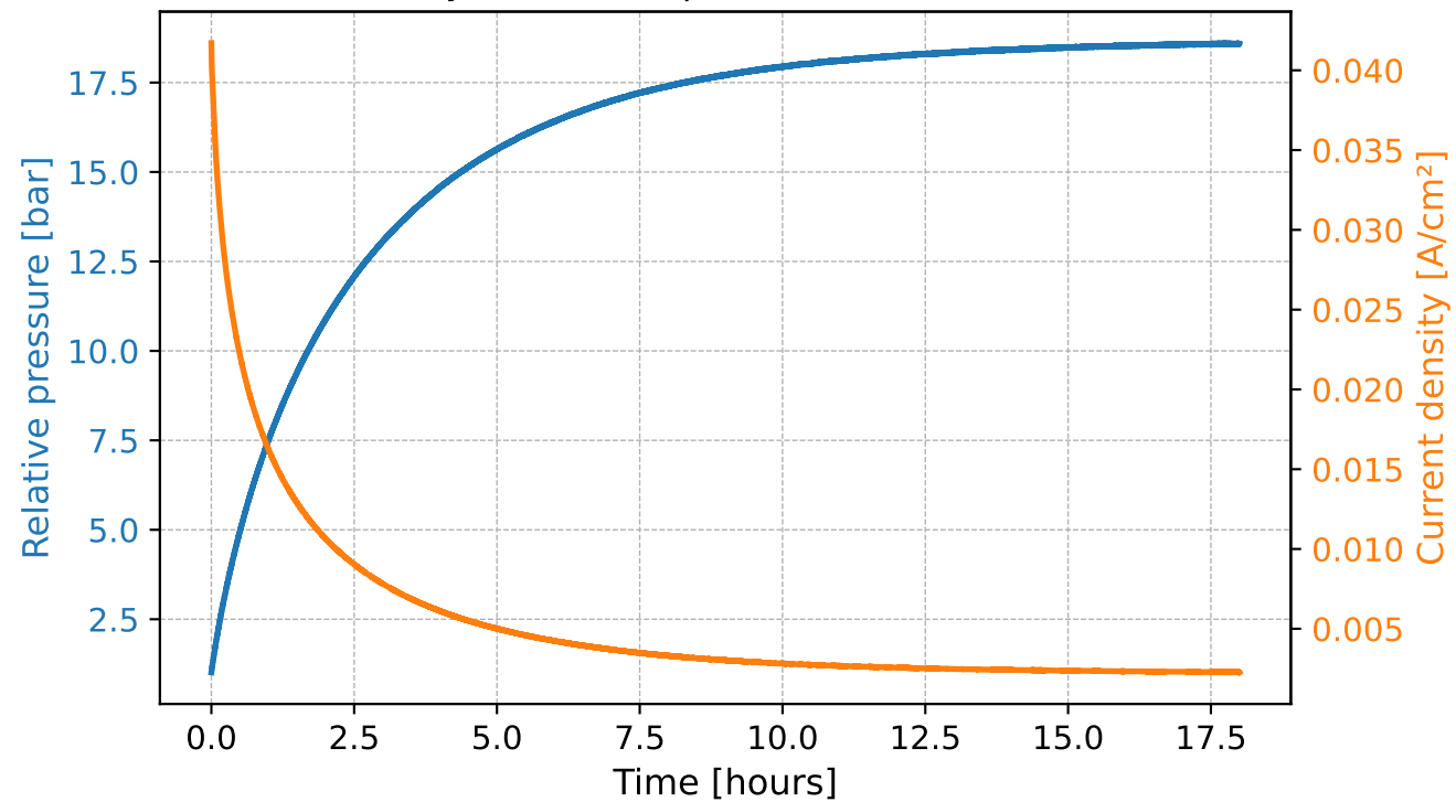
Current density vs Relative pressure of the cathode - 0.04 V
