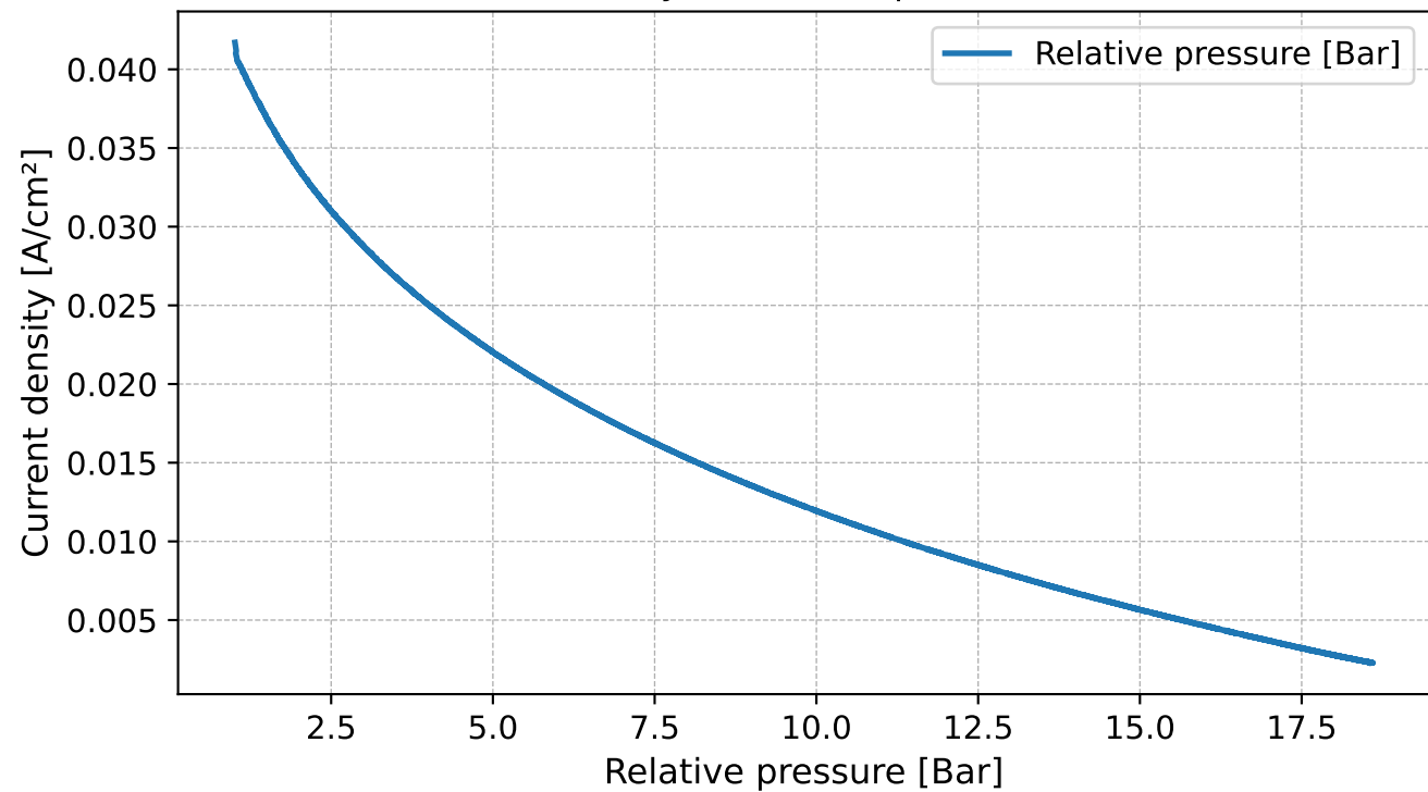
Current density vs Relative pressure - 0.04 V
