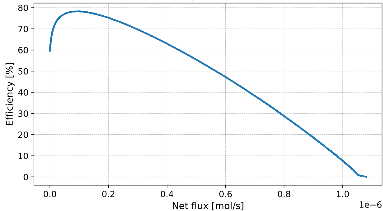
Work efficiency vs Net flux - 0.04 V
