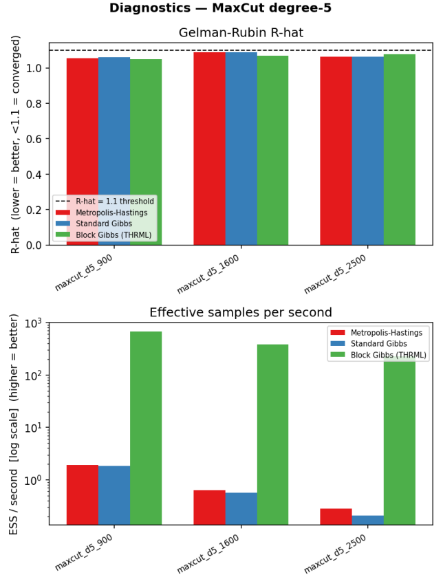
Fig. 6. Gelman-Rubin \hat{R} (top) and ESS/s on log scale (bottom) for MaxCut degree-5 across system sizes.
