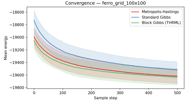
Fig. 2. Mean energy trace ( \pm 1 std across chains) for the 100 \times 100 ferromagnetic grid. All three samplers continue to descend throughout the sample window, indicating incomplete mixing within the sample budget.
