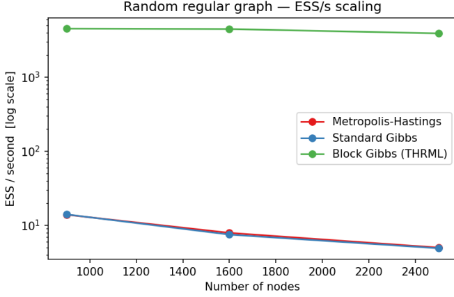
Fig. 5. ESS/s vs. number of nodes on log scale for the ferromagnetic RRG. THRML maintains two to three orders of magnitude higher throughput than MH and standard Gibbs at all sizes, while solution quality is statistically equivalent.
